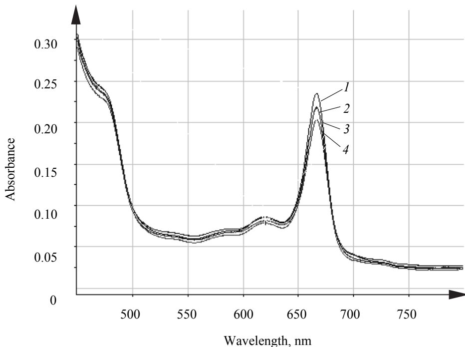
Fig. 2. Electronic absorption spectra of Chl in presence of Zn^{2+} : 1 – control; 2 – 1.96 \cdot 10^{-6} M ZnSO_4 ; 3 – 3.85 \cdot 10^{-6} M ZnSO_4 ; 4 – 5.65 \cdot 10^{-6} M ZnSO_4
