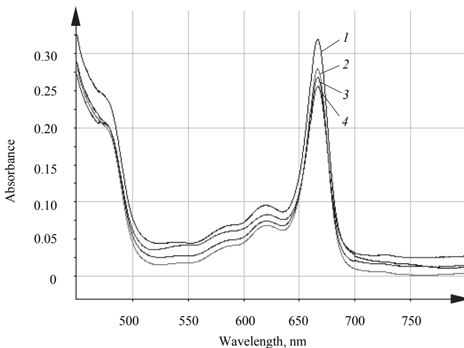
Fig. 3. Electronic absorption spectra of Chl in presence of Fe^{2+} : 1 – control; 2 – 1.96 \cdot 10^{-6} M FeSO_4 ; 3 – 3.85 \cdot 10^{-6} M FeSO_4 ; 4 – 5.65 \cdot 10^{-6} M FeSO_4
