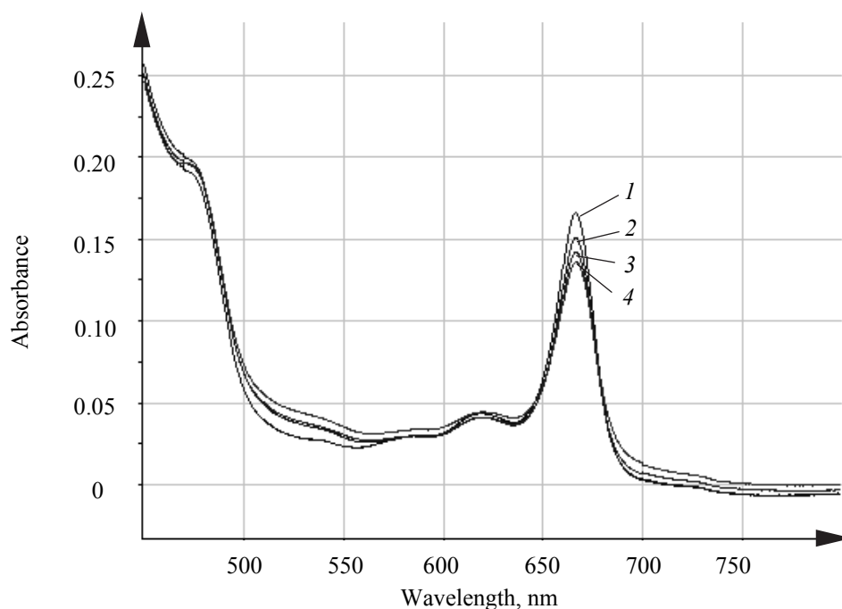
Fig. 1. Electronic absorption spectra of Chl in presence of \text{Cu}^{2+} :
