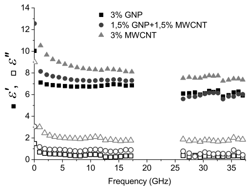
Figure 5. The complex permittivity of composites with 3 wt. % total filler content.
