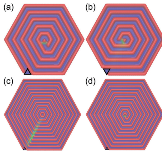
Fig. 7 Low temperature density maps of the system with different system sizes. Panels (a and b): M = 21 , panel (c): M = 44 , panel (d): M = 43 . The wedge position is marked by a black triangle and the color code is the same as in Fig. 5.
