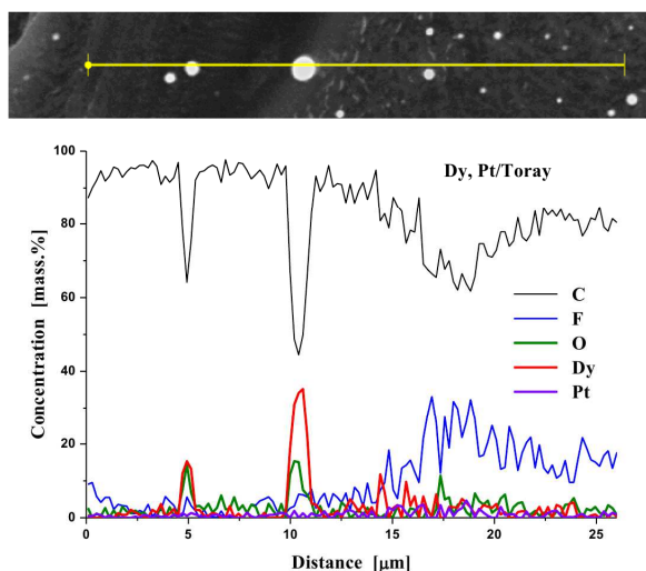
Fig. 1. Distribution of atoms of elements across the scanning line over the surface of Toray Carbon Fiber Paper TGP-H-060 T carrier with layer formed by the IBAD of dysprosium and platinum according EDX analysis.
