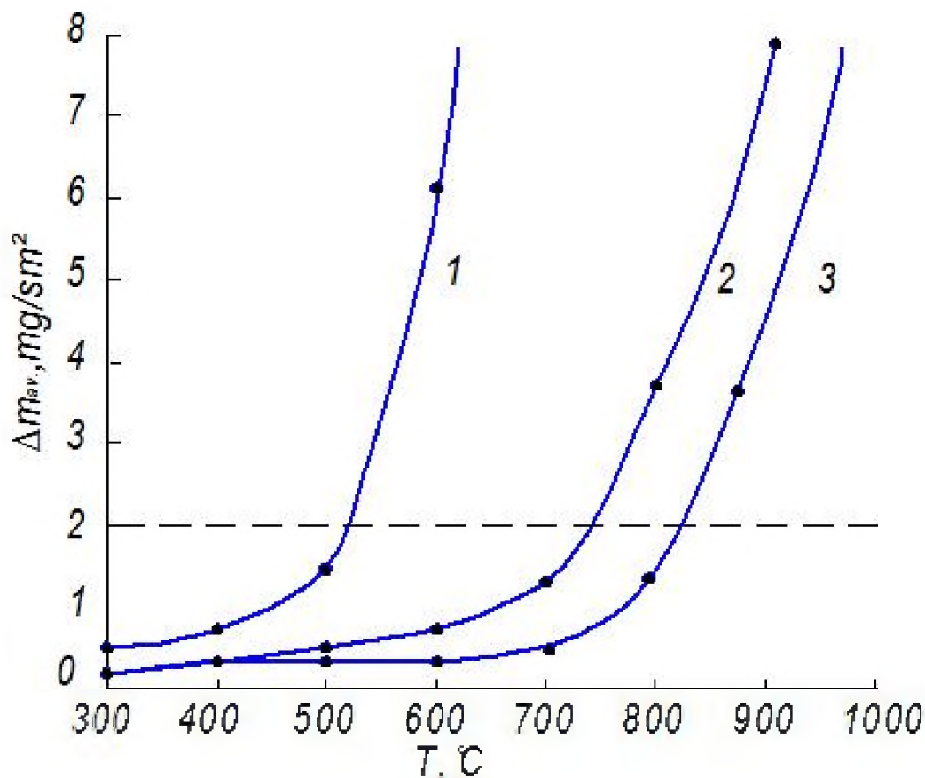
Fig. 5 - The mass increase of the vacuum arc coatings during heating in air under different aluminum concentrations
