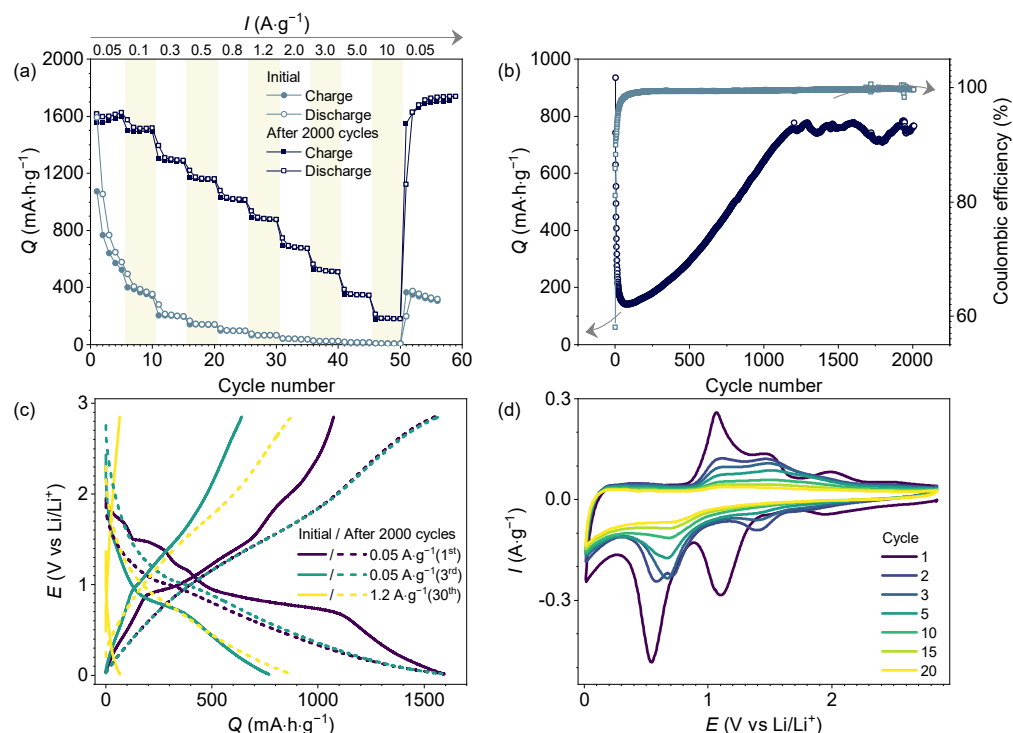
Figure 3. Electrochemical performance of FeOOH/PANI electrode: (a) C-rate capability; (b) cycling stability at I = 1.2 \text{ A} \cdot \text{g}^{-1} ; (c) charge/discharge curves during C-rate capability; (d) cyclic voltammograms at 0.1 \text{ mV} \cdot \text{s}^{-1} .
