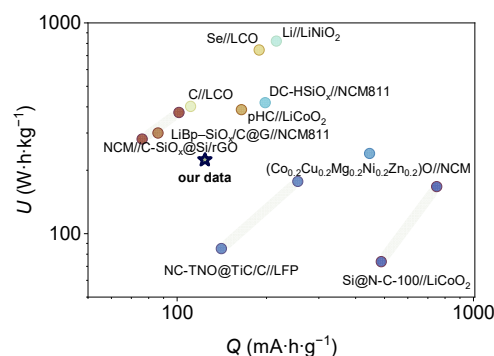
Figure 6. Comparison of NMC532//FeOOH/PANI full cell with other anodes in development: Si@N-C-100//LiCoO 2 [118], NC-TNO@TiC/C//LFP [119], NCM811//DC-HSiO x [120], Li//LiNiO 2 [121], LCO-Se [122], pHC/LiCoO 2 [123], LiBp-SiO x /C@G//NCM811 [124], NCM//C-SiO x @Si/rGO [125], and (\text{Co}_{0.2}\text{Cu}_{0.2}\text{Mg}_{0.2}\text{Ni}_{0.2}\text{Zn}_{0.2})\text{O} [117].
