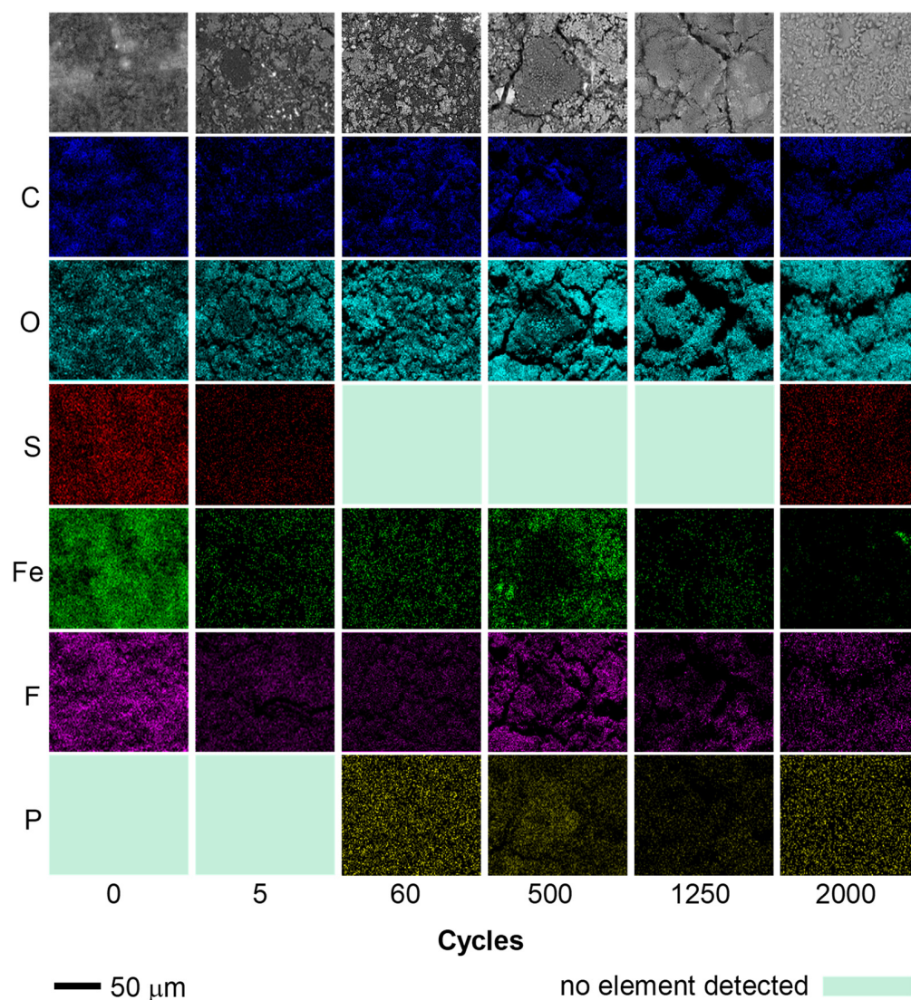
Figure 11. Element mapping for cycled electrodes obtained via EDX.
