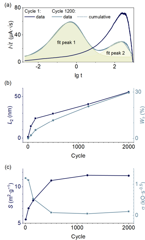
Figure 8. (a) Fitted Cottrell function plot for the current transient versus the decimal logarithm for 1st and 1200th cycles; (b) dependence of particle size L_2 and its mass content on the cycle number; (c) correlation between specific surface area from PITT and Warburg constant from EIS.
