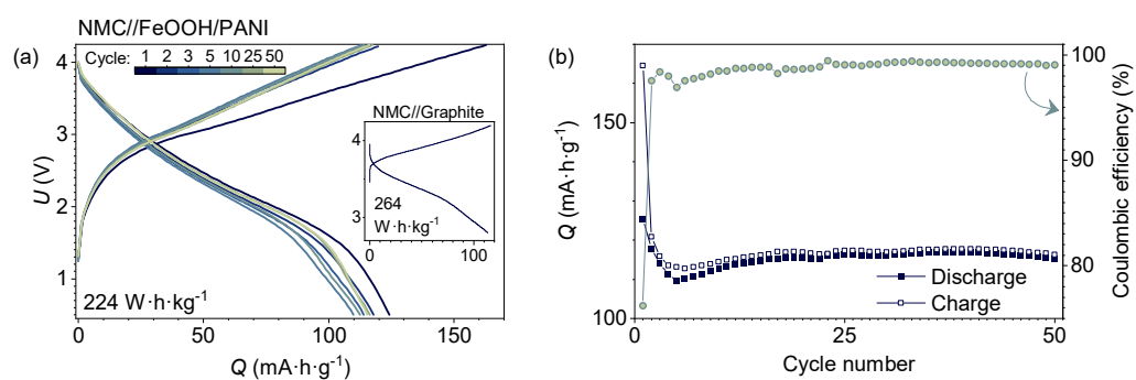
Figure 5. NMC532//FeOOH/PANI full cell performance within the (0.5–4.20) V range at C/2 referred to the NMC532 cathode mass (1 C = 140 mA·g -1 ) in terms of (a) selected voltage profiles, inset : charge–discharge curve of the NMC532//Graphite full cell at a C/2 rate; (b) trends of specific capacity and coulombic efficiency. Electrolyte: 1 M LiPF 6 in EC/DEC (1:1, v/v).
