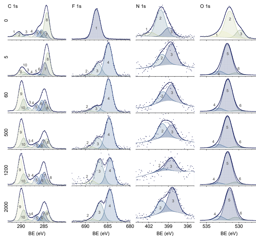
Figure 10. XPS spectra of C 1s, F 1s, N 1s, and O 1s for FeOOH/PANI electrode after cycling. The rows are for cycle numbers 0, 5, 60, 500, 1200, and 2000, and the columns are for the C, F, N, and O 1s bands. In each spectrum, dark blue dots are for experimental data, thick blue line is approximation curve, and dotted gray line is background curve. Fitted peaks assignment: in C 1s: 1—C-F ( \text{C}_n\text{F}_m ) \pi - \pi^* , 2—C-F (PVDF), 3—R-F (organoflourine), 4—C=O, 5—C-OH/C-N + -C/CH 2 -CH 2 (PVDF), 6—C-N-C/C-O-C, 7—C=C ( \text{sp}^2 ), 8—C-C ( \text{sp}^3 ), 9— \text{Li}_2\text{CO}_3 , 10—O=C-O; in F 1s: 1—C-F (PVDF), 2—LiF, 3— \text{Li}_x\text{PO}_y-1\text{F}_{z+1} , 4—C-F ( \text{C}_n\text{F}_m ); in N 1s: 1—positively charged nitrogen (oxidized amine), 2—benzenoid amine (-NH-), 3—imine (-N=); in O 1s: 1— \text{SO}_4^{2-} , 2—Fe-OH, 3—Fe=O, 4—C-O-C/P-O-P, 5—C=O/P=O/-OH, 6—Fe in the oxide matrix.
