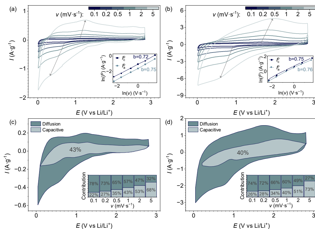
Figure 4. FeOOH/PANI after 20 cycles: (a) CVs at various scan rates; inset shows \ln(I_{\text{peak}}) vs. \ln(v) plot; (c) pseudocapacitance contribution to total capacity at 1 \text{ mV}\cdot\text{s}^{-1} , inset shows contribution ratios of capacitive and diffusion-controlled currents at various scan rates. FeOOH/PANI after 2000 cycles: (b) CVs at various scan rates; inset shows \ln(I_{\text{peak}}) vs. \ln(v) plot; (d) pseudocapacitance contribution to total capacity at 1 \text{ mV}\cdot\text{s}^{-1} , inset shows contribution ratios of capacitive and diffusion-controlled currents at various scan rates.
