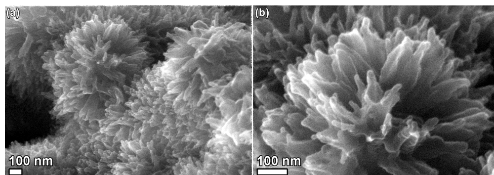
Figure 1. (a,b) FeOOH/PANI SEM images at different magnification.
