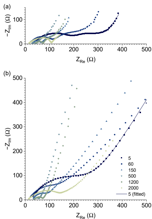
Figure 7. Impedance spectra of the cells with FeOOH electrodes at intermediate points during long-term cycling at OCV (a) after discharge and (b) after charge.
