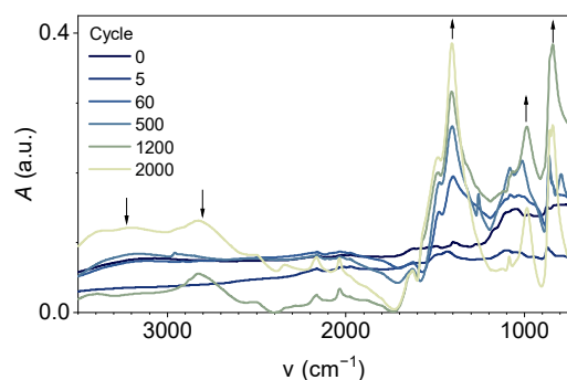
Figure 9. ATR-FTIR spectra of FeOOH/PANI electrodes after different number of recharging cycles.
