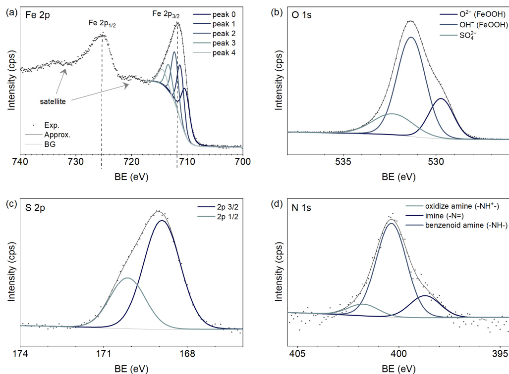
Figure 2. XPS spectra of FeOOH/PANI: (a) Fe 2p; (b) O 1s; (c) S 2p; (d) N 1s.
